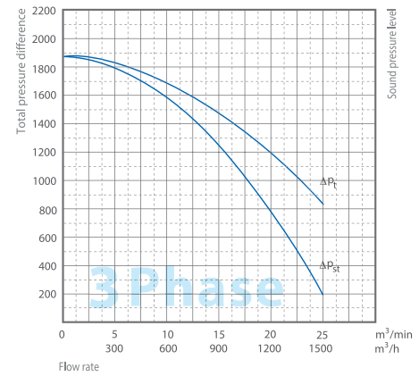
MSS-55A/T
