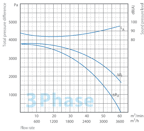
MSR-60A/T
