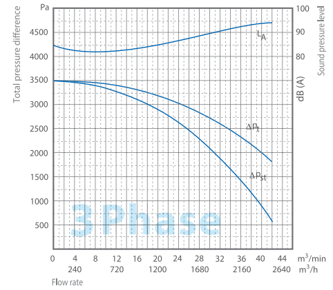
MSR-50B/T
