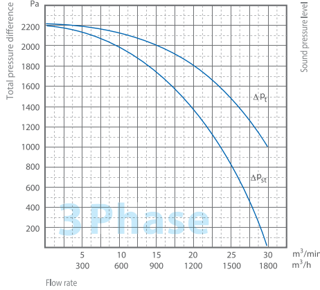
MSS-55B/T
