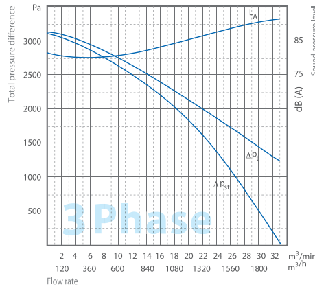
MSR-50A/T
