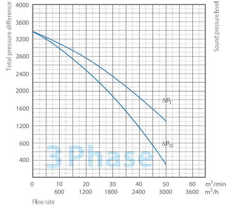
MSS-65A/T
