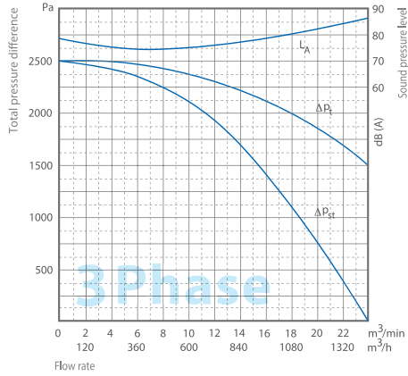
MSR-40B/T
