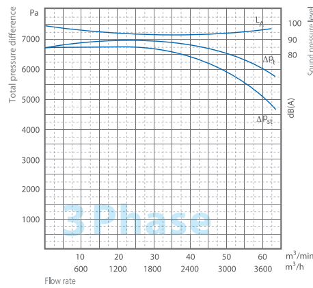
MSR-70B/T
